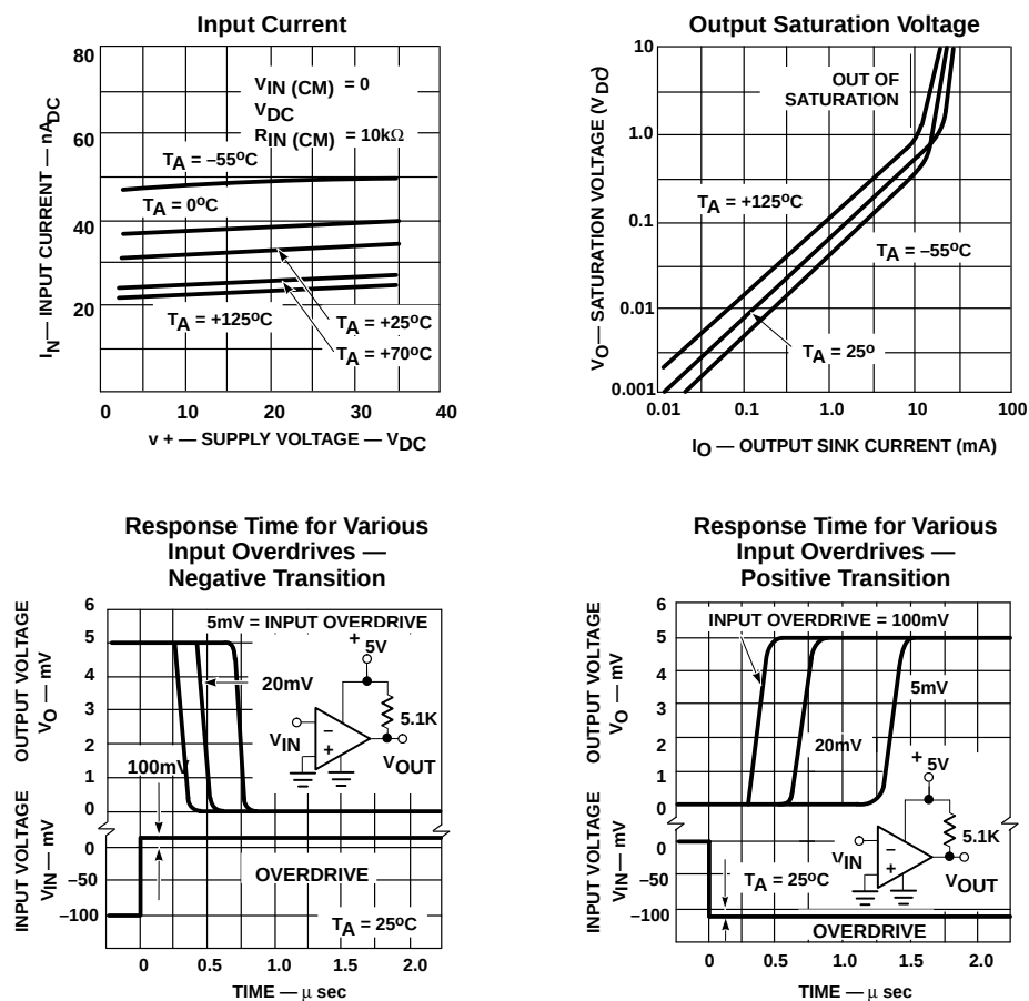
Figure 4. Typical Performance Characteristics
